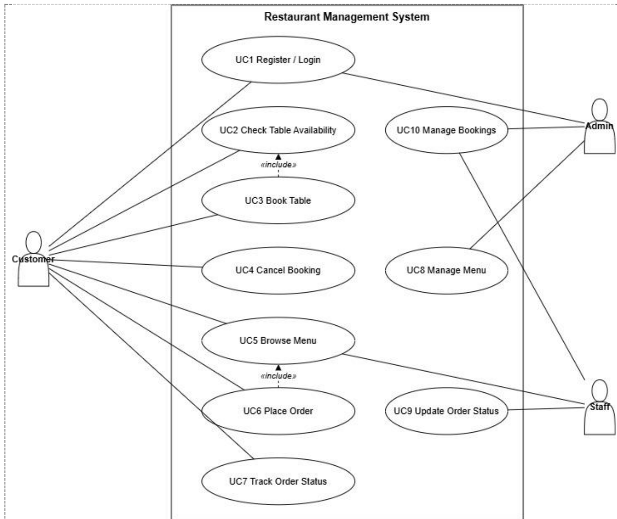
Figure 1: UML use case diagram for the Restaurant Management System
